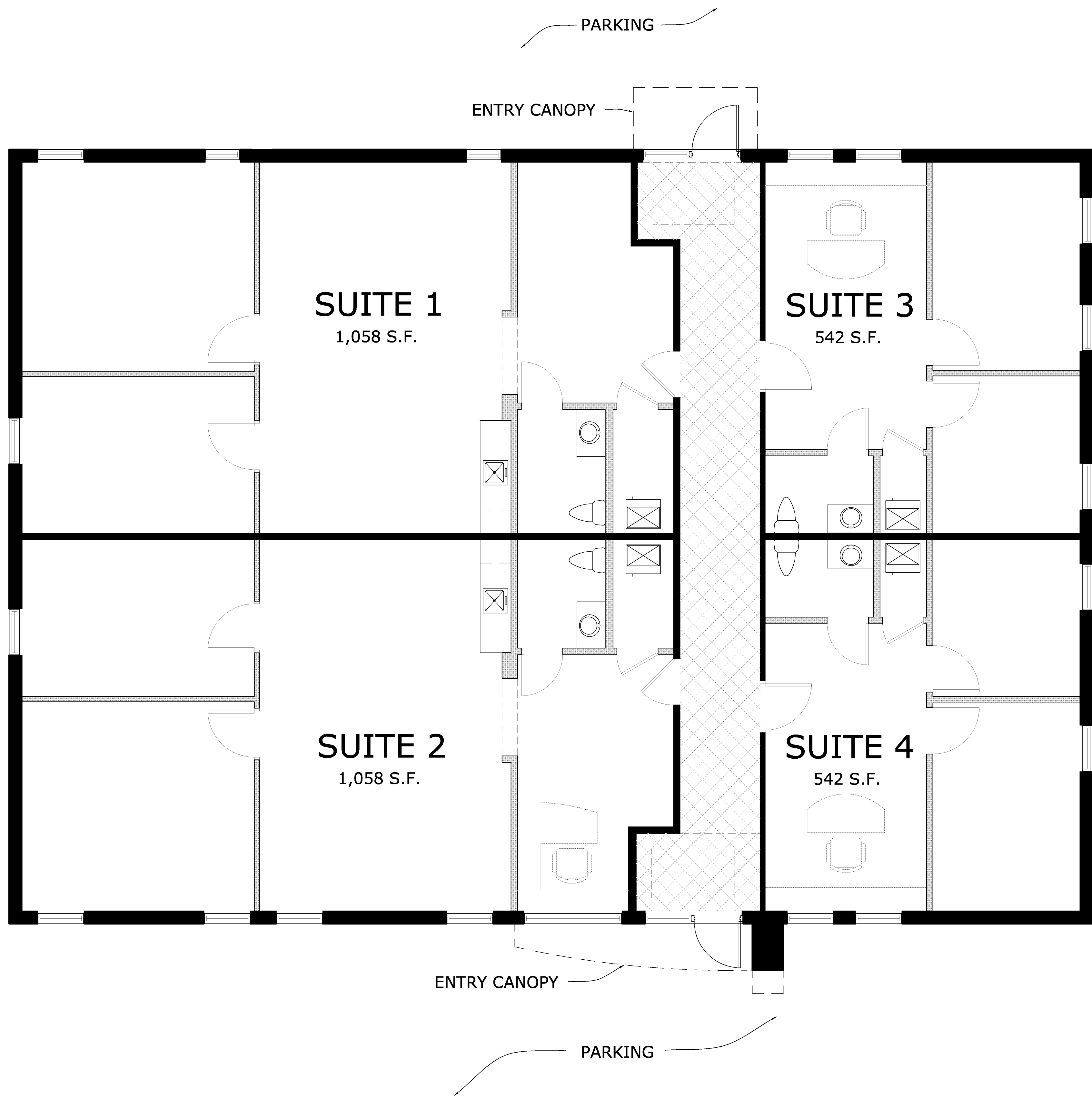
FLOOR PLAN
